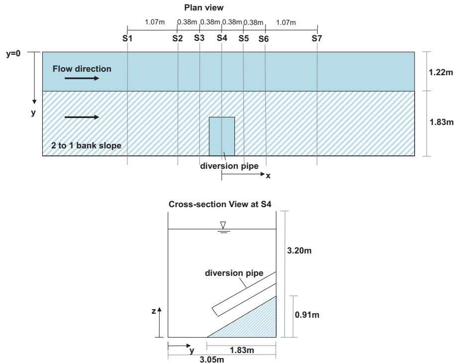
FIGURE 3. Main Flow Direction Components ( x , y , z directions) and the Measurement Cross Sections.
