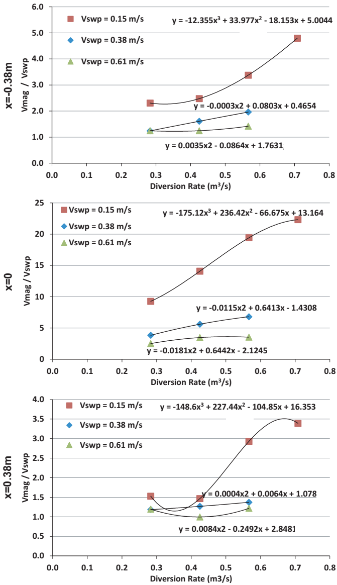
FIGURE 9. Maximum Values of Nondimensional Velocity Magnitudes V_{mag}/V_{swp} for Various Diversion Rates at x = -0.38, 0, 0.38 m (scales of y-axis are different for each figure).
