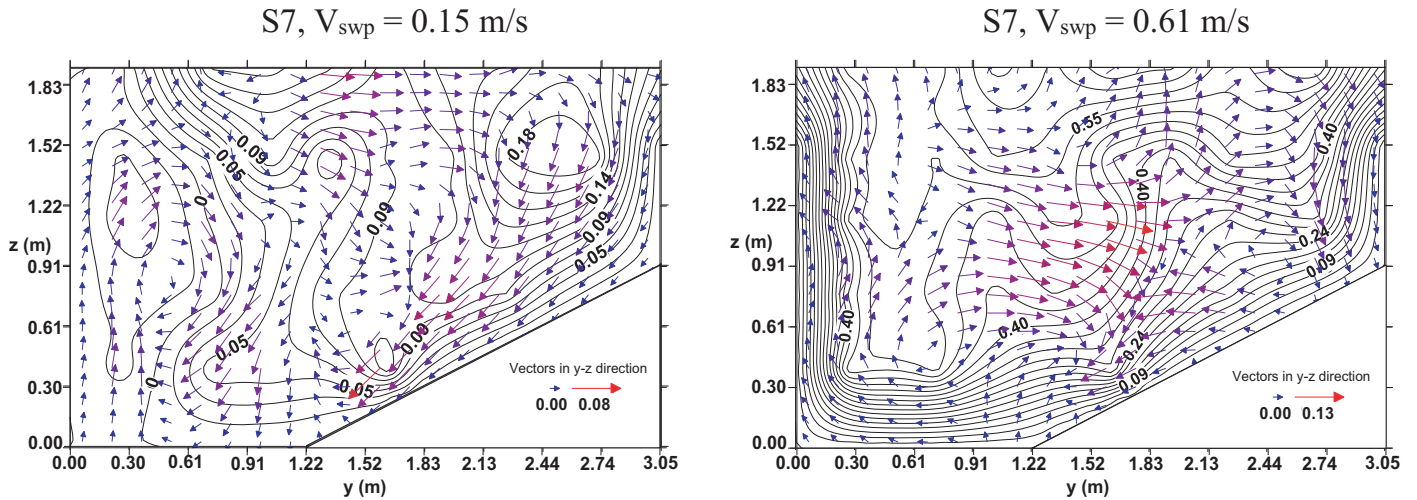
FIGURE 6. Contours of x-Direction Velocities Superimposed on Velocity Vectors of y- and z-Directions at Cross Section S7 for 0.15 and 0.61 m/s Sweeping Velocities with a 0.57 \text{ m}^3/\text{s} Diversion Rate (i.e., figures for Test 5 on the left and Test 7 on the right).
