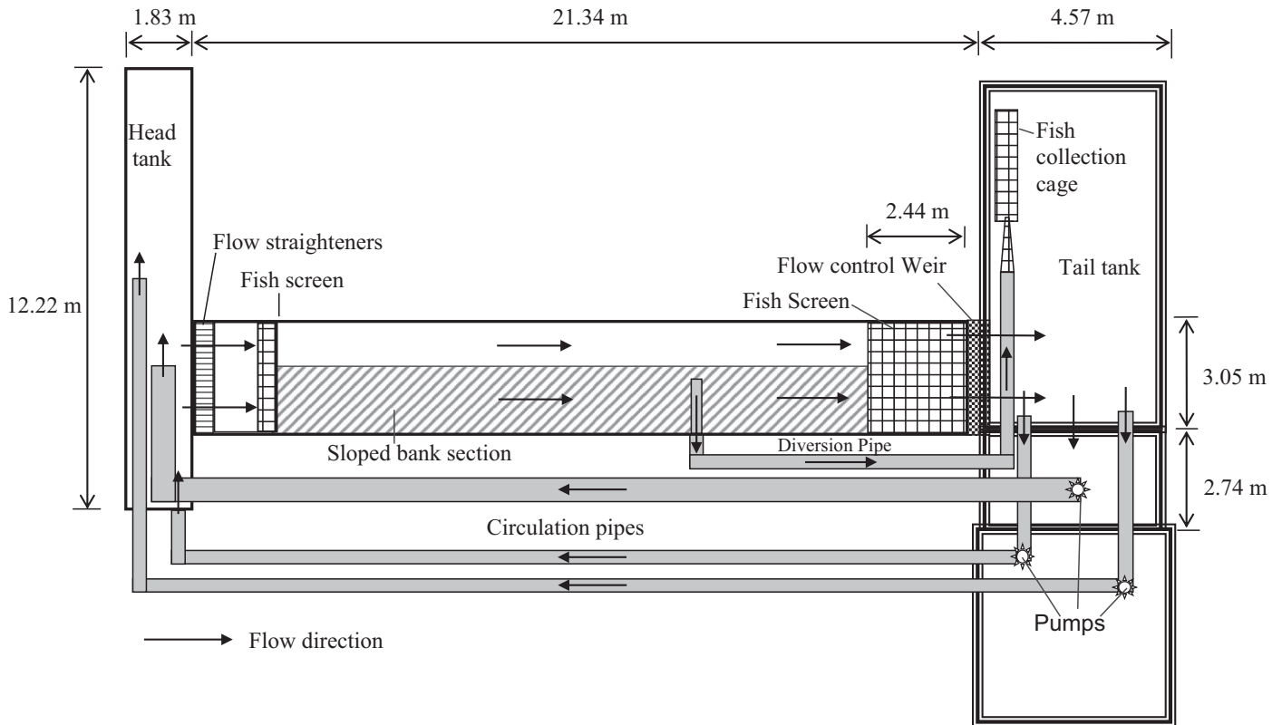
FIGURE 1. Plan View of Experimental Flume Setup.
