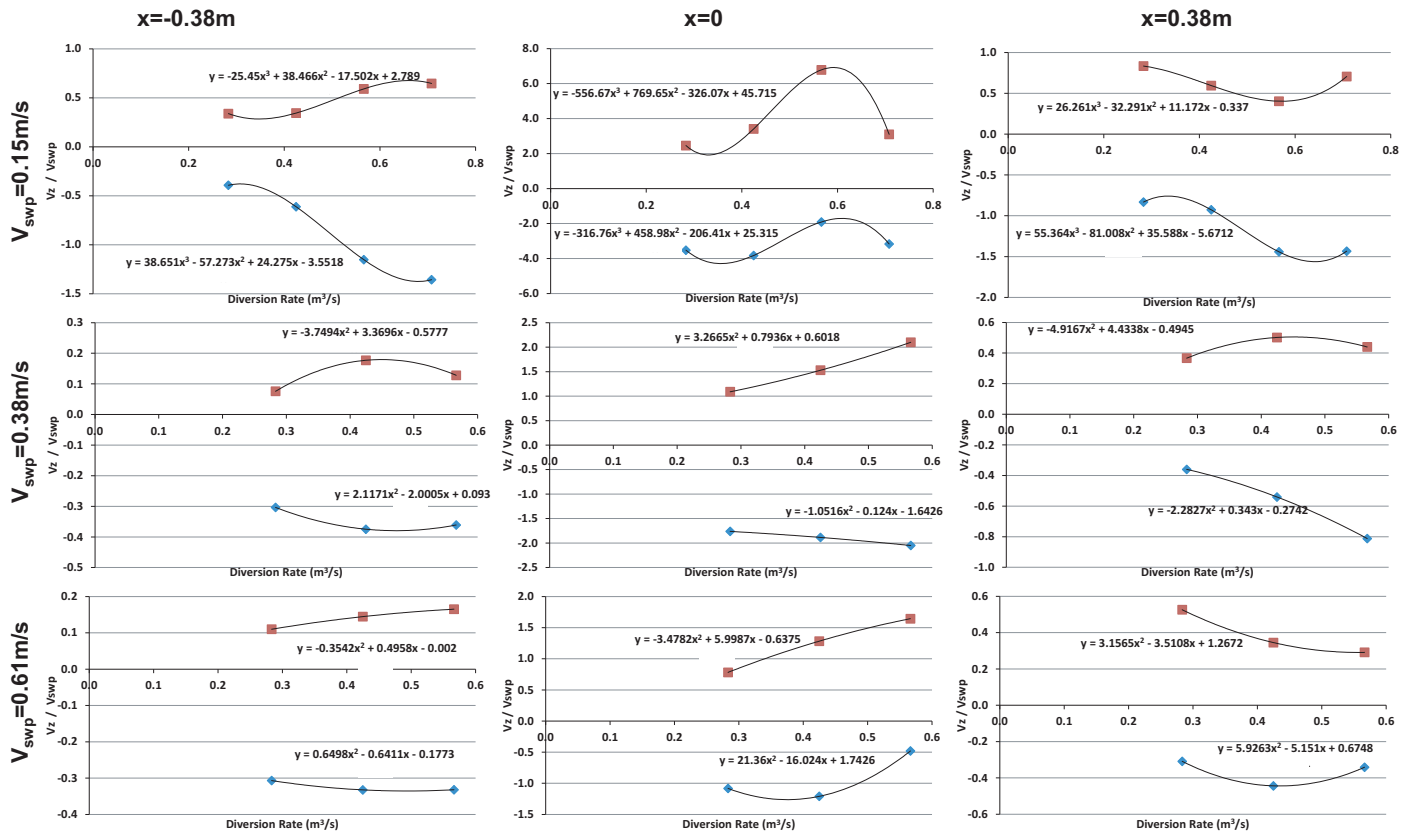
FIGURE 8. Maximum Values of Positive and Negative Nondimensional z -Direction Velocity V_z/V_{swp} for Various Diversion Rates and Sweeping Velocities at x = -0.38, 0, 0.38 m (scales of y -axis are different for each figure).
