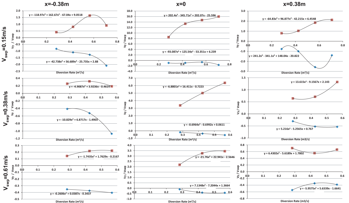
FIGURE 7. Maximum Values of Positive and Negative Nondimensional Transverse (y-) Direction Velocities V_y/V_{swp} for Various Diversion Rates and Sweeping Velocities at x = -0.38, 0, 0.38 \text{ m} (scales of y-axis are different for each figure).
